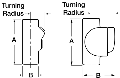
ENY Series
